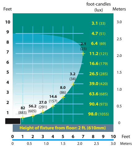
FFL-5 Half Spread Photometrics
