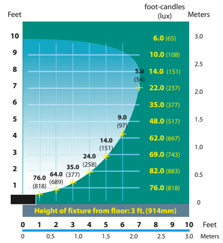
FFL-9 Half Spread Photometrics
