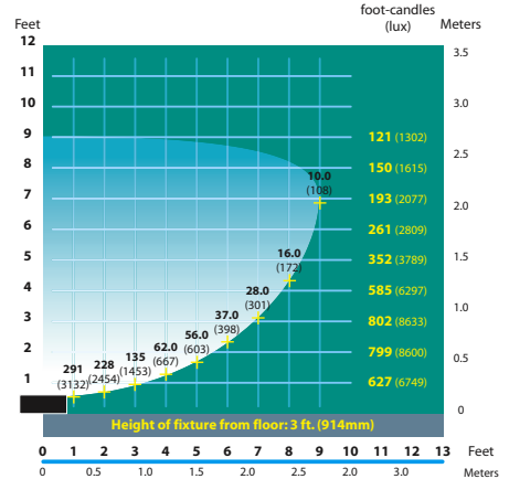
FFL-39T5HO Half Spread Photometrics
