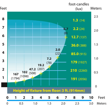
FFL-13-HE Half Spread Photometrics
