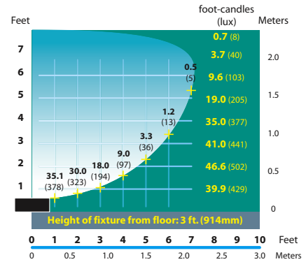
FFL-5-HE Half Spread Photometrics
