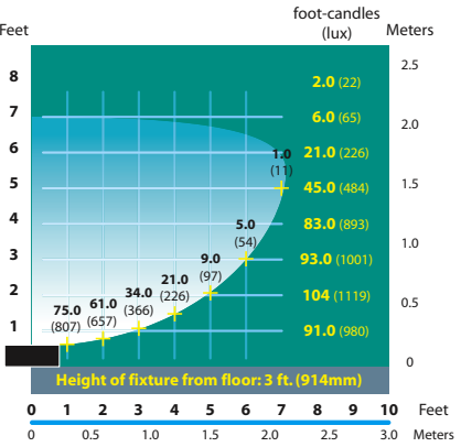
FFL-9-HE Half Spread Photometrics
