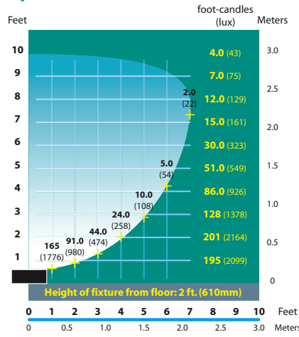
FFL-9 Half Spread Photometrics
