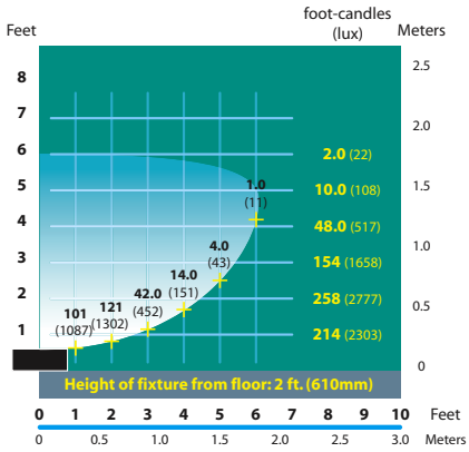
FFL-9-HE Half Spread Photometrics
