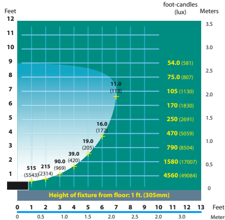
FFL-39T5HO Half Spread Photometrics
