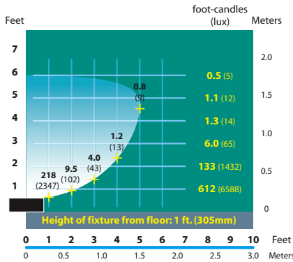
FFL-5-HE Half Spread Photometrics
