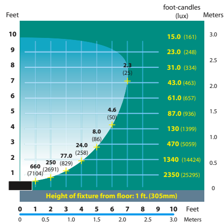
FFL-26-HE ON FA-26 2 x 13w Lamp (26w max.) Extruded Aluminum
