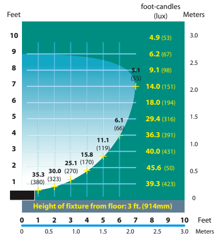
FFL-5 Half Spread Photometrics
